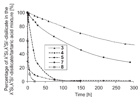
Figure 11. Kinetics of the hydrolysis of 3–5 and 7–8 upon dissolution in \text{D}_2\text{O} (10 mM; pH 6.4 \pm 0.2 ( 3 ), 5.6 \pm 0.2 ( 4 ), 5.5 \pm 0.2 ( 5 ), 6.2 \pm 0.2 ( 7 ), 5.9 \pm 0.2 ( 8 )). The experimental data were extracted from ^1\text{H} NMR spectra (23 °C, 500.1 MHz) in which the CH resonance signals of the zwitterionic \lambda^5\text{Si},\lambda^5\text{Si}' -disilicates and free ( R,R )-tartaric acid served as the probe. The pH values given were measured directly after sample preparation.
